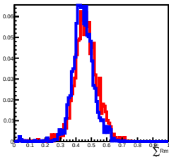
Deposit Energy[10.00GeV, 15.85GeV] in L10
