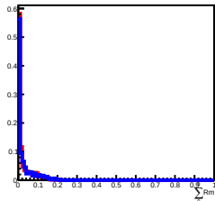
Deposit Energy[10.00GeV, 15.85GeV] in L5
