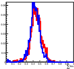
Deposit Energy[10.00GeV, 15.85GeV] in L9
