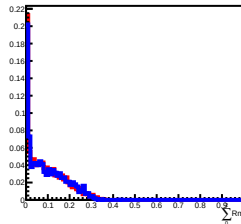
Deposit Energy[25.12GeV, 39.81GeV] in L7
