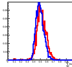
Deposit Energy[25.12GeV, 39.81GeV] in L12
