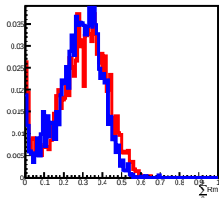
Deposit Energy[25.12GeV, 39.81GeV] in L10
