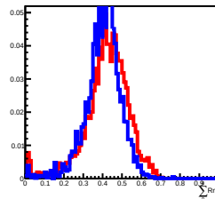
Deposit Energy[25.12GeV, 39.81GeV] in L13
