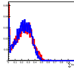
Deposit Energy[25.12GeV, 39.81GeV] in L9
