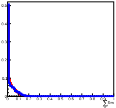
Deposit Energy[39.81GeV, 63.10GeV] in L6
