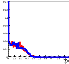
Deposit Energy[39.81GeV, 63.10GeV] in L8
