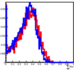
Deposit Energy[63.10GeV, 100.00GeV] in L11
