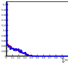
Deposit Energy[63.10GeV, 100.00GeV] in L8
