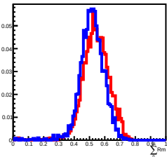
Deposit Energy[63.10GeV, 100.00GeV] in L11
