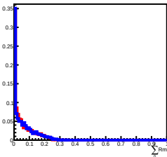
Deposit Energy[63.10GeV, 100.00GeV] in L7
