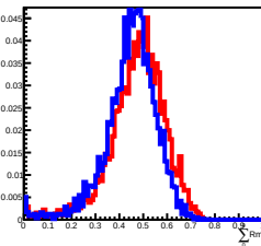
Deposit Energy[63.10GeV, 100.00GeV] in L9
