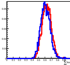
Deposit Energy[100.00GeV, 158.49GeV] in L13
