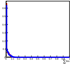
Deposit Energy[100.00GeV, 158.49GeV] in L6
