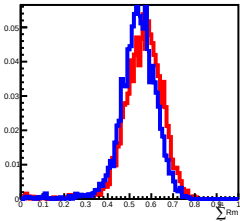
Deposit Energy[100.00GeV, 158.49GeV] in L11
