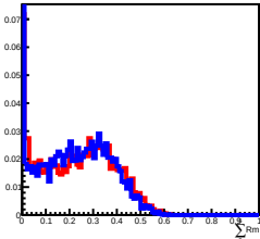
Deposit Energy[100.00GeV, 158.49GeV] in L10
