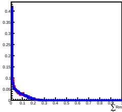
Deposit Energy[100.00GeV, 158.49GeV] in L7
