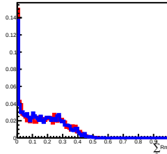
Deposit Energy[100.00GeV, 158.49GeV] in L9
