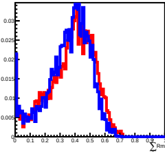
Deposit Energy[100.00GeV, 158.49GeV] in L12
