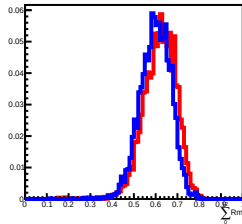
Deposit Energy[158.49GeV, 251.19GeV] in L12
