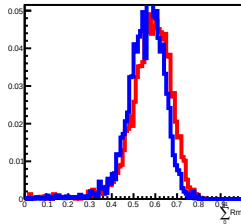
Deposit Energy[158.49GeV, 251.19GeV] in L11
