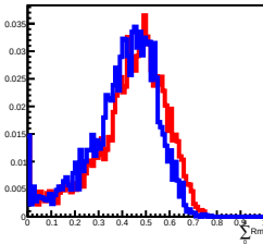
Deposit Energy[158.49GeV, 251.19GeV] in L13
