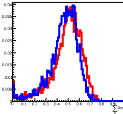
Deposit Energy[158.49GeV, 251.19GeV] in L9
