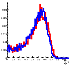
Deposit Energy[1000.00GeV, 1584.89GeV] in L9
