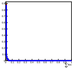
Deposit Energy[1000.00GeV, 1584.89GeV] in L6
