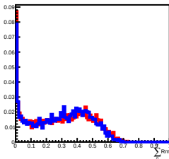
Deposit Energy[1000.00GeV, 1584.89GeV] in L12
