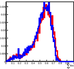
Deposit Energy[1000.00GeV, 1584.89GeV] in L10
