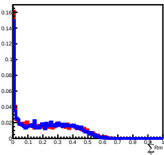
Deposit Energy[1000.00GeV, 1584.89GeV] in L11
