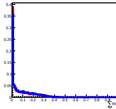
Deposit Energy[1000.00GeV, 1584.89GeV] in L9
