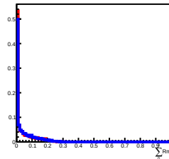
Deposit Energy[1000.00GeV, 1584.89GeV] in L8
