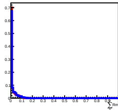
Deposit Energy[1000.00GeV, 1584.89GeV] in L7
