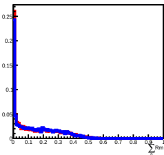
Deposit Energy[1000.00GeV, 1584.89GeV] in L10
