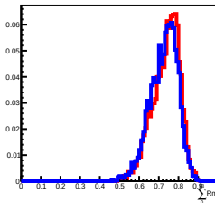
Deposit Energy[1000.00GeV, 1584.89GeV] in L13
