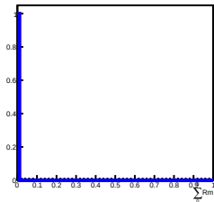
Deposit Energy[1000.00GeV, 1584.89GeV] in L5
