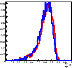
Deposit Energy[1000.00GeV, 1584.89GeV] in L11
