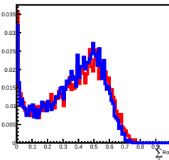
Deposit Energy[1000.00GeV, 1584.89GeV] in L13
