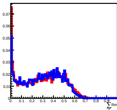
Deposit Energy[1584.89GeV, 2511.89GeV] in L12
