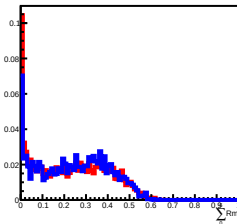
Deposit Energy[2511.89GeV, 3981.07GeV] in L11
