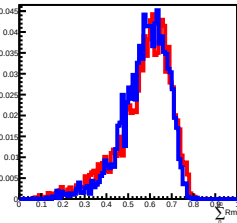
Deposit Energy[2511.89GeV, 3981.07GeV] in L10
