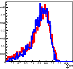
Deposit Energy[2511.89GeV, 3981.07GeV] in L9
