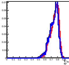
Deposit Energy[2511.89GeV, 3981.07GeV] in L13
