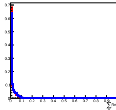
Deposit Energy[2511.89GeV, 3981.07GeV] in L7
