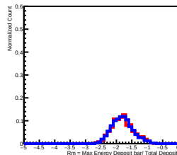
Deposit Energy[10.00GeV, 15.85GeV] in L9
