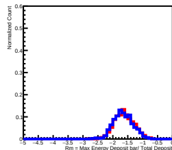
Deposit Energy[10.00GeV, 15.85GeV] in L7
