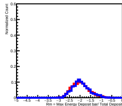
Deposit Energy[10.00GeV, 15.85GeV] in L12
