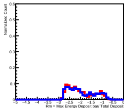
Deposit Energy[10.00GeV, 15.85GeV] in L0
