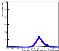
Deposit Energy[10.00GeV, 15.85GeV] in L10
