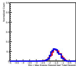
Deposit Energy[10.00GeV, 15.85GeV] in L6
