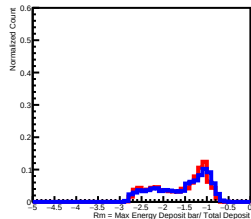
Deposit Energy[10.00GeV, 15.85GeV] in L1
