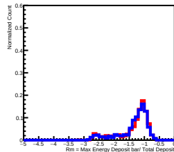
Deposit Energy[10.00GeV, 15.85GeV] in L2
