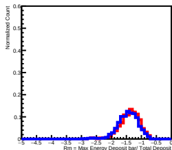
Deposit Energy[10.00GeV, 15.85GeV] in L5
