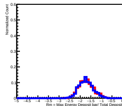
Deposit Energy[10.00GeV, 15.85GeV] in L8
