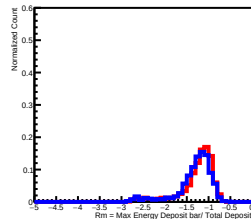
Deposit Energy[10.00GeV, 15.85GeV] in L3
