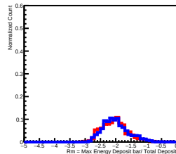
Deposit Energy[10.00GeV, 15.85GeV] in L13
