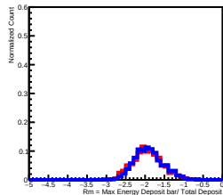
Deposit Energy[10.00GeV, 15.85GeV] in L11
