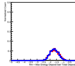
Deposit Energy[15.85GeV, 25.12GeV] in L8
