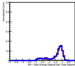
Deposit Energy[15.85GeV, 25.12GeV] in L2
