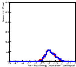
Deposit Energy[15.85GeV, 25.12GeV] in L11
