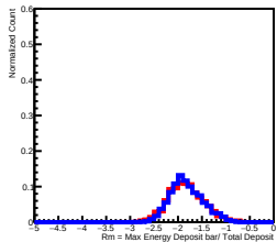
Deposit Energy[15.85GeV, 25.12GeV] in L10
