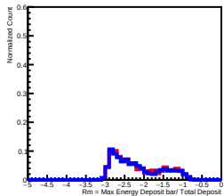
Deposit Energy[15.85GeV, 25.12GeV] in L0
