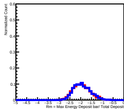
Deposit Energy[15.85GeV, 25.12GeV] in L12
