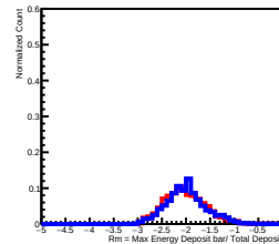
Deposit Energy[15.85GeV, 25.12GeV] in L13
