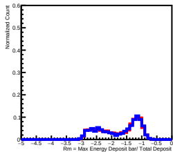
Deposit Energy[15.85GeV, 25.12GeV] in L1
