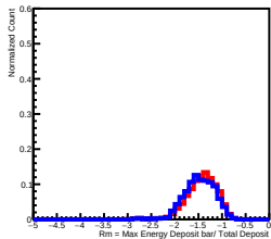
Deposit Energy[15.85GeV, 25.12GeV] in L6
