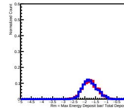
Deposit Energy[15.85GeV, 25.12GeV] in L9
