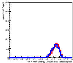
Deposit Energy[15.85GeV, 25.12GeV] in L5
