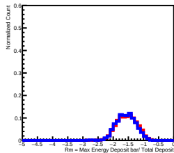
Deposit Energy[15.85GeV, 25.12GeV] in L7
