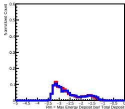
Deposit Energy[39.81GeV, 63.10GeV] in L0
