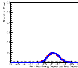
Deposit Energy[39.81GeV, 63.10GeV] in L12
