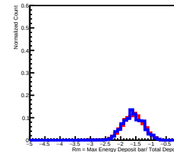
Deposit Energy[39.81GeV, 63.10GeV] in L9
