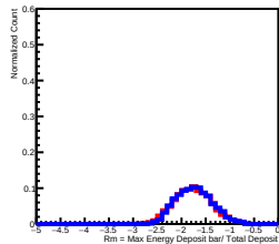
Deposit Energy[39.81GeV, 63.10GeV] in L11
