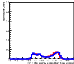
Deposit Energy[39.81GeV, 63.10GeV] in L1
