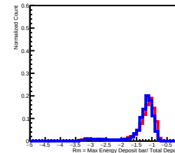
Deposit Energy[39.81GeV, 63.10GeV] in L4
