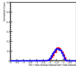
Deposit Energy[39.81GeV, 63.10GeV] in L7
