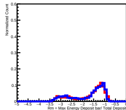
Deposit Energy[39.81GeV, 63.10GeV] in L2
