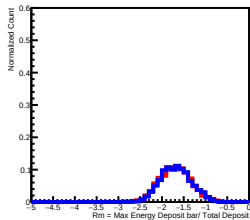
Deposit Energy[39.81GeV, 63.10GeV] in L10
