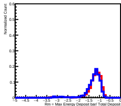
Deposit Energy[39.81GeV, 63.10GeV] in L5
