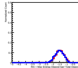
Deposit Energy[39.81GeV, 63.10GeV] in L8
