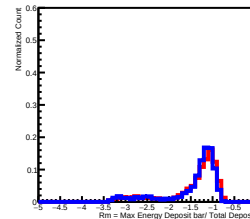
Deposit Energy[39.81GeV, 63.10GeV] in L3
