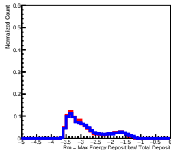
Deposit Energy[63.10GeV, 100.00GeV] in L0
