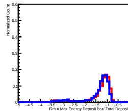
Deposit Energy[63.10GeV, 100.00GeV] in L4
