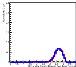
Deposit Energy[63.10GeV, 100.00GeV] in L7
