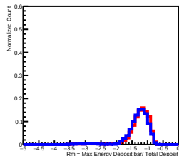
Deposit Energy[63.10GeV, 100.00GeV] in L6
