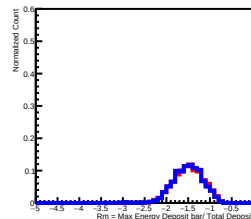
Deposit Energy[63.10GeV, 100.00GeV] in L9
