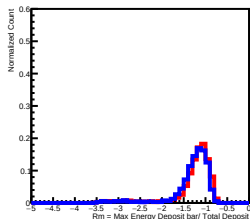
Deposit Energy[63.10GeV, 100.00GeV] in L5
