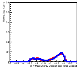
Deposit Energy[63.10GeV, 100.00GeV] in L2
