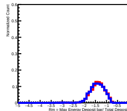
Deposit Energy[63.10GeV, 100.00GeV] in L8
