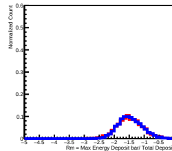
Deposit Energy[398.11GeV, 630.96GeV] in L13
