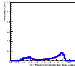
Deposit Energy[398.11GeV, 630.96GeV] in L3
