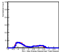
Deposit Energy[398.11GeV, 630.96GeV] in L1
