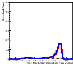
Deposit Energy[398.11GeV, 630.96GeV] in L5
