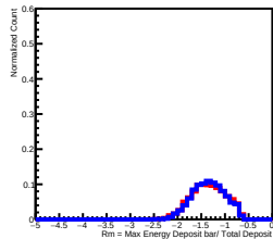
Deposit Energy[398.11GeV, 630.96GeV] in L11
