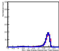
Deposit Energy[398.11GeV, 630.96GeV] in L6
