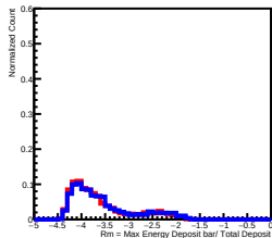
Deposit Energy[398.11GeV, 630.96GeV] in L0
