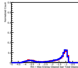
Deposit Energy[398.11GeV, 630.96GeV] in L4
