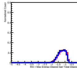
Deposit Energy[398.11GeV, 630.96GeV] in L9
