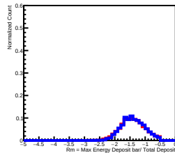
Deposit Energy[398.11GeV, 630.96GeV] in L12
