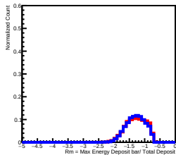
Deposit Energy[398.11GeV, 630.96GeV] in L10
