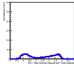
Deposit Energy[398.11GeV, 630.96GeV] in L2
