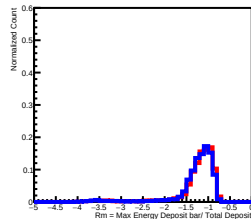
Deposit Energy[398.11GeV, 630.96GeV] in L7
