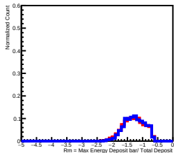
Deposit Energy[630.96GeV, 1000.00GeV] in L11
