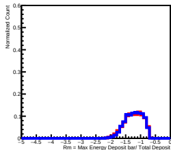
Deposit Energy[630.96GeV, 1000.00GeV] in L10
