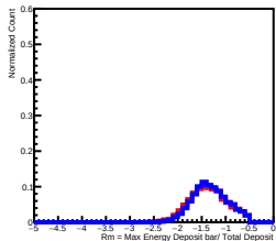
Deposit Energy[630.96GeV, 1000.00GeV] in L12
