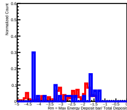
Deposit Energy(6309.57GeV, 10000.00GeV) in L2
