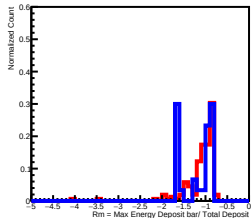
Deposit Energy(6309.57GeV, 10000.00GeV) in L5
