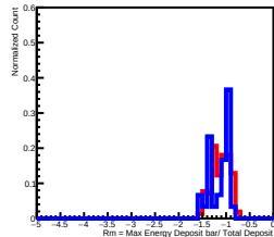
Deposit Energy(6309.57GeV, 10000.00GeV) in L9
