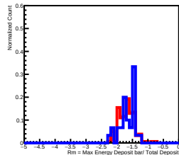
Deposit Energy(6309.57GeV, 10000.00GeV) in L12
