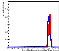
Deposit Energy(6309.57GeV, 10000.00GeV) in L7
