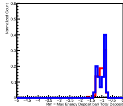
Deposit Energy(6309.57GeV, 10000.00GeV) in L8
