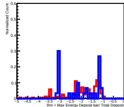
Deposit Energy(6309.57GeV, 10000.00GeV) in L3
