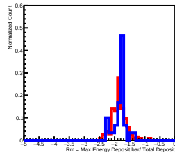
Deposit Energy(6309.57GeV, 10000.00GeV) in L13
