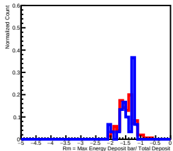
Deposit Energy(6309.57GeV, 10000.00GeV) in L11
