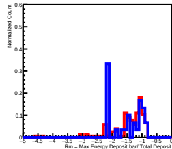
Deposit Energy(6309.57GeV, 10000.00GeV) in L4
