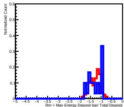
Deposit Energy(6309.57GeV, 10000.00GeV) in L10
