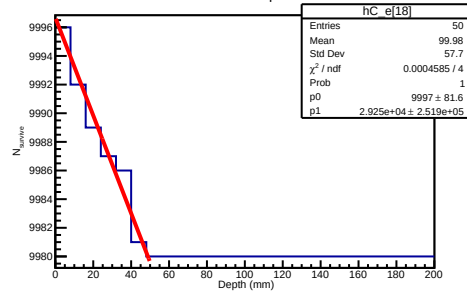
1000 GeV Electron Depth Distribution
