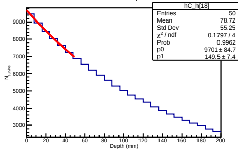
1000 GeV Helium4 Depth Distribution
