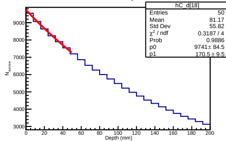
1000 GeV Deuteron Depth Distribution
