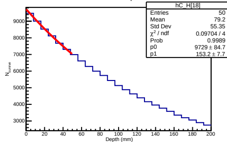
1000 GeV Helium3 Depth Distribution
