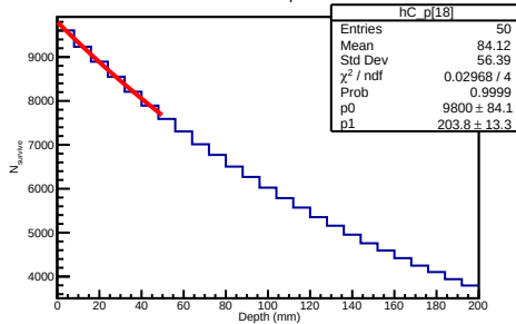
1000 GeV Proton Depth Distribution
