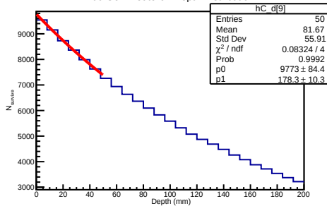
100 GeV Deuteron Depth Distribution
