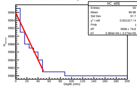
100 GeV Electron Depth Distribution
