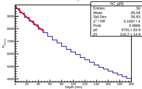
100 GeV Proton Depth Distribution
