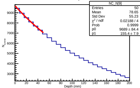
100 GeV Helium4 Depth Distribution
