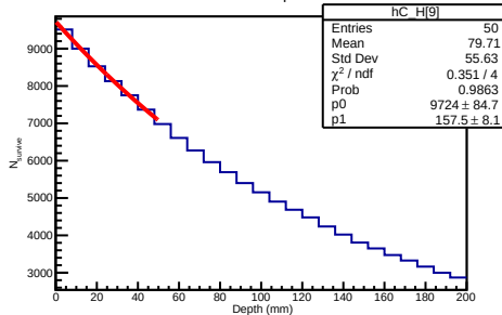
100 GeV Helium3 Depth Distribution
