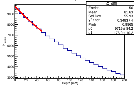
10 GeV Deuteron Depth Distribution
