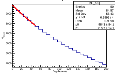
10 GeV Proton Depth Distribution
