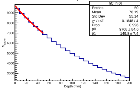
10 GeV Helium4 Depth Distribution
