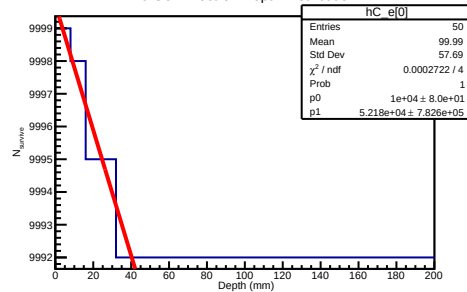
10 GeV Electron Depth Distribution
