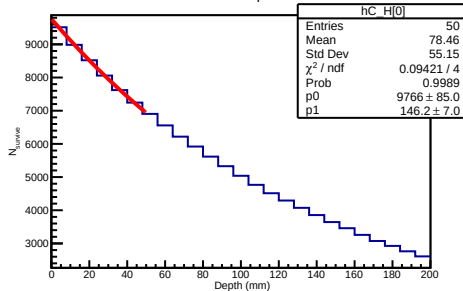
10 GeV Helium3 Depth Distribution
