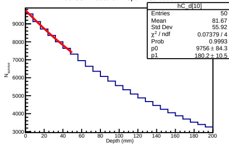
200 GeV Deuteron Depth Distribution
