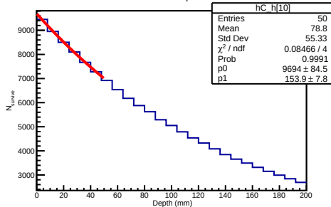
200 GeV Helium4 Depth Distribution
