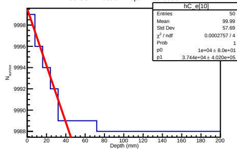
200 GeV Electron Depth Distribution
