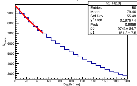
200 GeV Helium3 Depth Distribution
