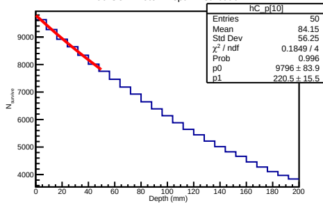
200 GeV Proton Depth Distribution
