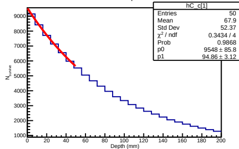
20 GeV Carbon Depth Distribution
