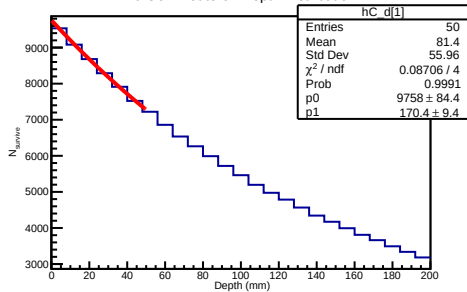
20 GeV Deuteron Depth Distribution
