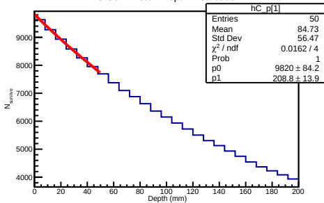
20 GeV Proton Depth Distribution
