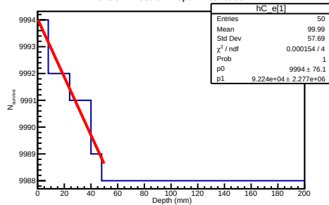
20 GeV Electron Depth Distribution
