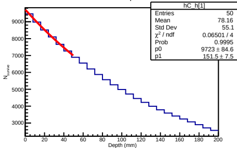
20 GeV Helium4 Depth Distribution
