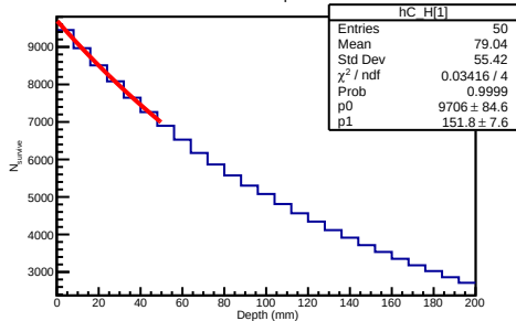
20 GeV Helium3 Depth Distribution
