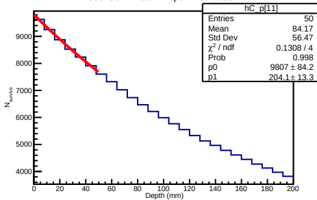
300 GeV Proton Depth Distribution
