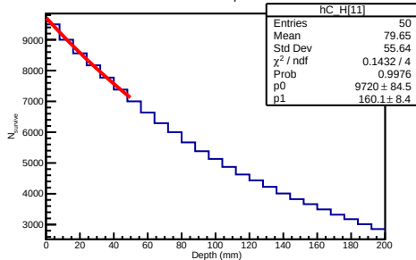
300 GeV Helium3 Depth Distribution
