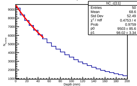
300 GeV Carbon Depth Distribution
