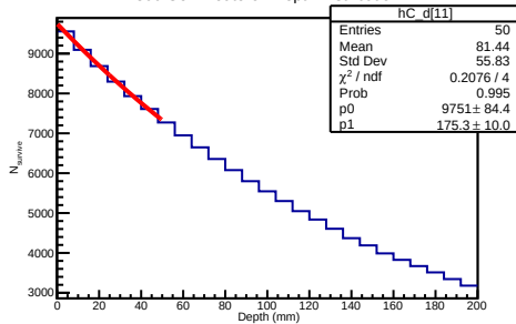
300 GeV Deuteron Depth Distribution
