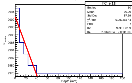
300 GeV Electron Depth Distribution
