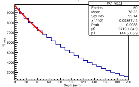
300 GeV Helium4 Depth Distribution
