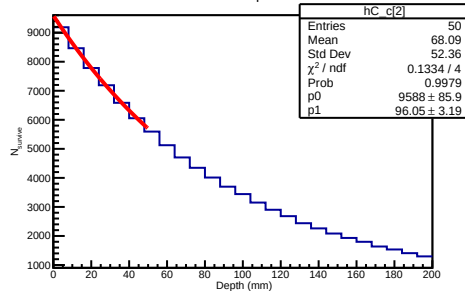
30 GeV Carbon Depth Distribution
