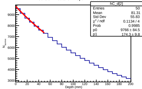
30 GeV Deuteron Depth Distribution
