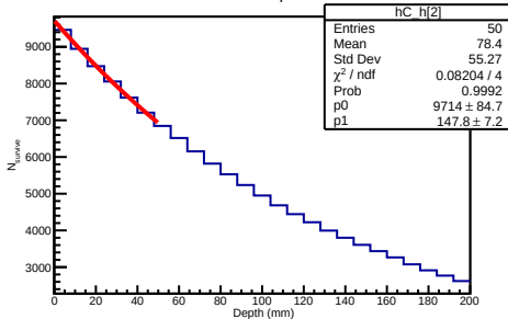
30 GeV Helium4 Depth Distribution
