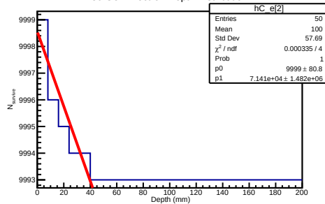
30 GeV Electron Depth Distribution
