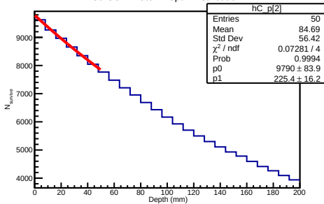
30 GeV Proton Depth Distribution
