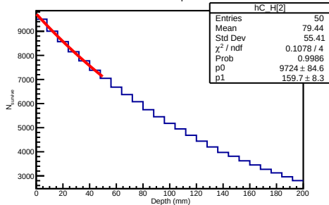
30 GeV Helium3 Depth Distribution
