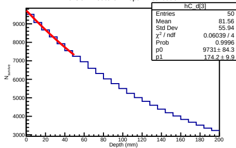
40 GeV Deuteron Depth Distribution
