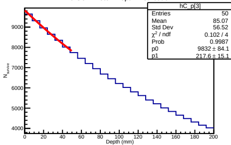
40 GeV Proton Depth Distribution
