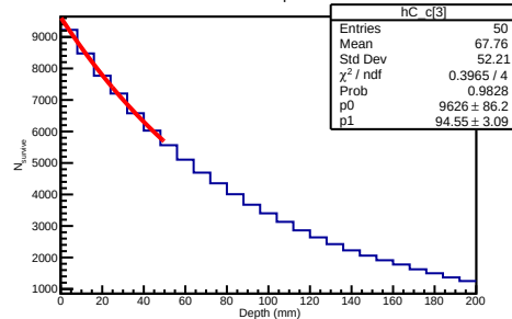
40 GeV Carbon Depth Distribution
