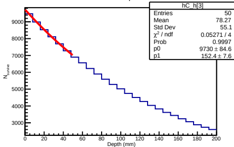
40 GeV Helium4 Depth Distribution
