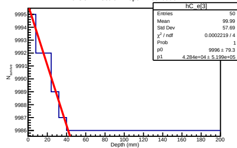
40 GeV Electron Depth Distribution
