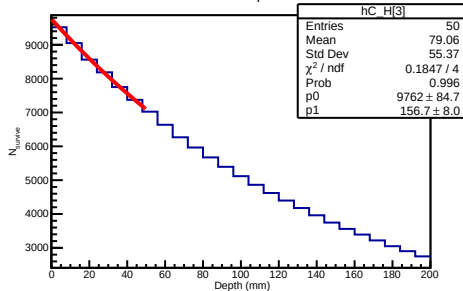
40 GeV Helium3 Depth Distribution
