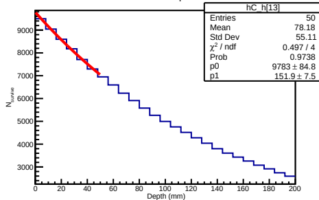
500 GeV Helium4 Depth Distribution
