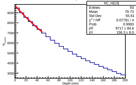
500 GeV Helium3 Depth Distribution
