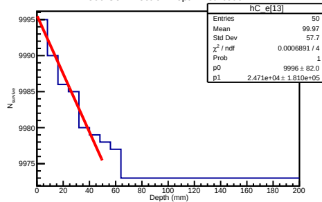
500 GeV Electron Depth Distribution
