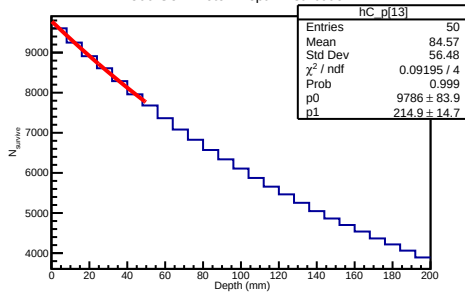
500 GeV Proton Depth Distribution
