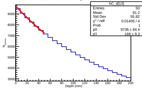
500 GeV Deuteron Depth Distribution
