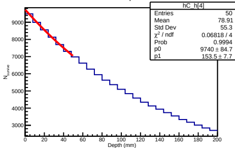
50 GeV Helium4 Depth Distribution
