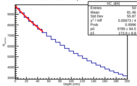
50 GeV Deuteron Depth Distribution
