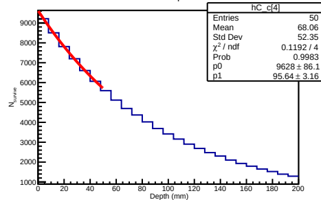
50 GeV Carbon Depth Distribution
