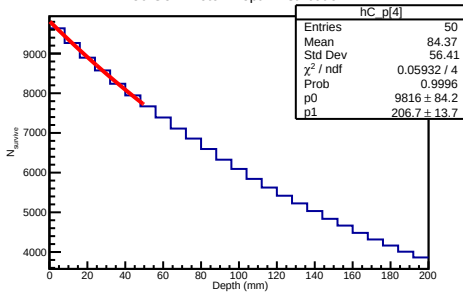
50 GeV Proton Depth Distribution
