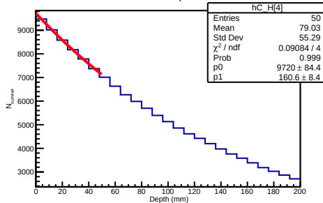
50 GeV Helium3 Depth Distribution
