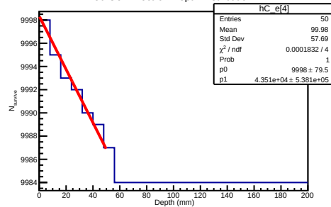
50 GeV Electron Depth Distribution
