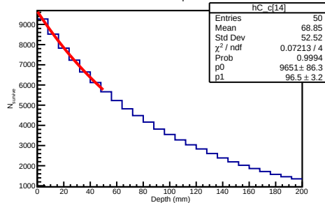
600 GeV Carbon Depth Distribution
