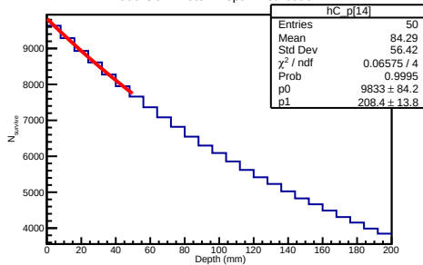
600 GeV Proton Depth Distribution
