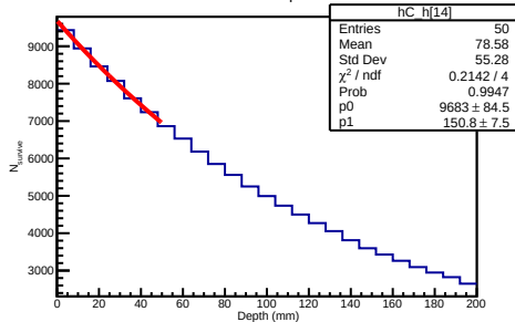
600 GeV Helium4 Depth Distribution
