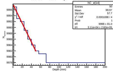
600 GeV Electron Depth Distribution
