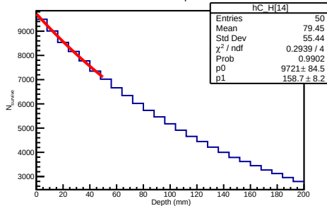
600 GeV Helium3 Depth Distribution
