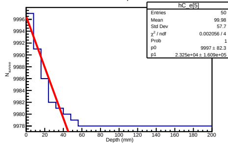
60 GeV Electron Depth Distribution
