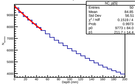
60 GeV Proton Depth Distribution
