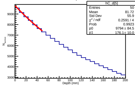
60 GeV Deuteron Depth Distribution
