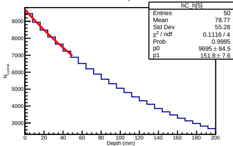
60 GeV Helium4 Depth Distribution
