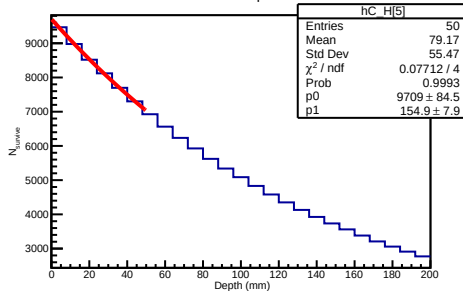
60 GeV Helium3 Depth Distribution
