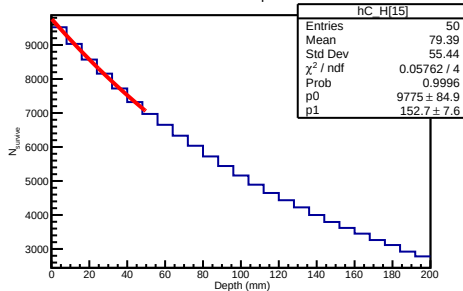
700 GeV Helium3 Depth Distribution
