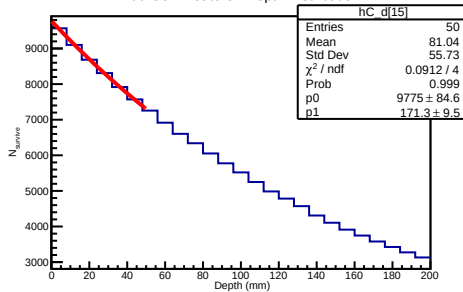
700 GeV Deuteron Depth Distribution
