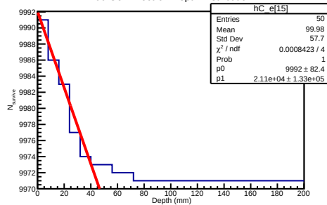
700 GeV Electron Depth Distribution
