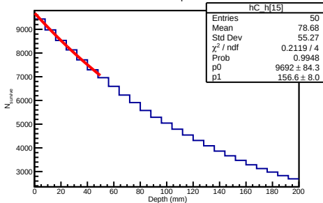
700 GeV Helium4 Depth Distribution
