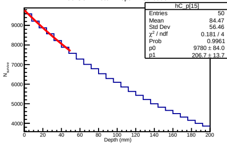
700 GeV Proton Depth Distribution
