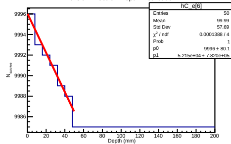
70 GeV Electron Depth Distribution
