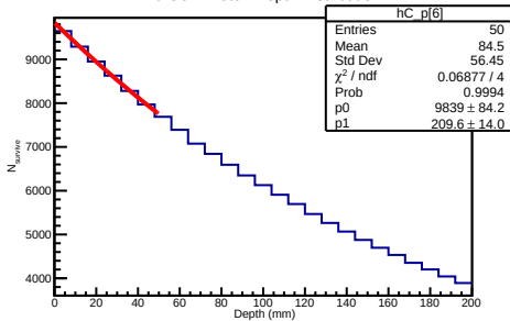
70 GeV Proton Depth Distribution
