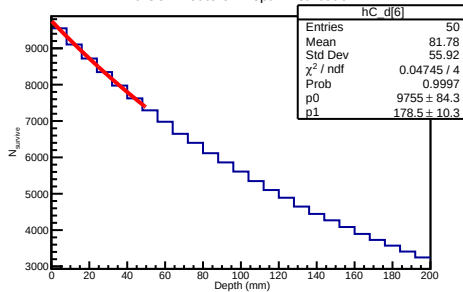
70 GeV Deuteron Depth Distribution
