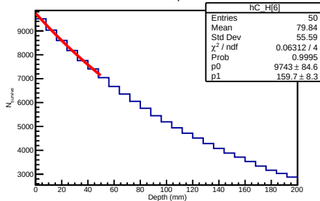
70 GeV Helium3 Depth Distribution
