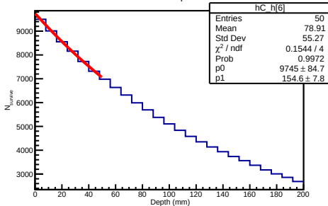
70 GeV Helium4 Depth Distribution
