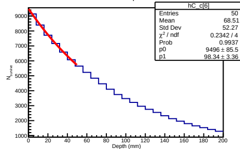
70 GeV Carbon Depth Distribution
