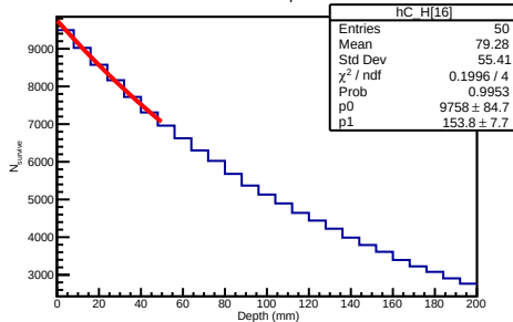
800 GeV Helium3 Depth Distribution
