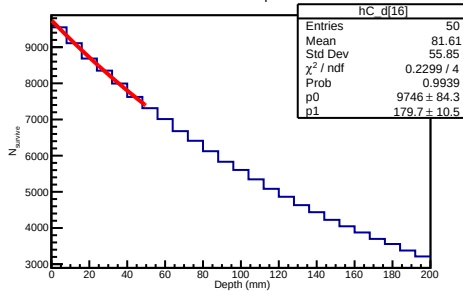
800 GeV Deuteron Depth Distribution
