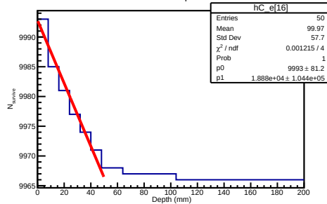
800 GeV Electron Depth Distribution
