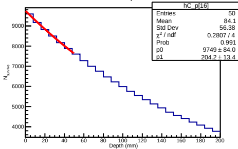
800 GeV Proton Depth Distribution
