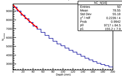
800 GeV Helium4 Depth Distribution
