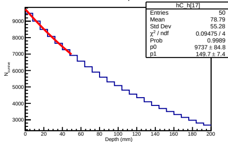
900 GeV Helium4 Depth Distribution
