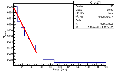
900 GeV Electron Depth Distribution
