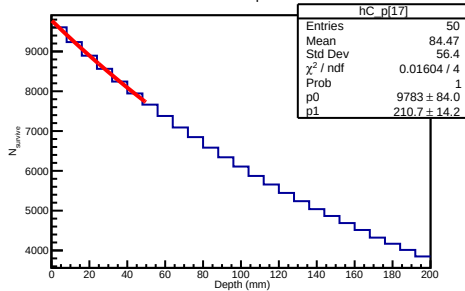
900 GeV Proton Depth Distribution
