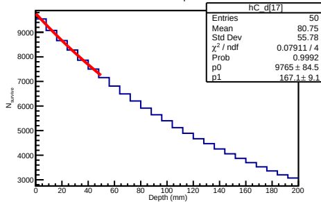
900 GeV Deuteron Depth Distribution
