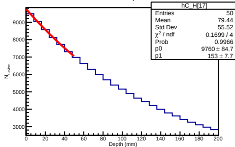
900 GeV Helium3 Depth Distribution
