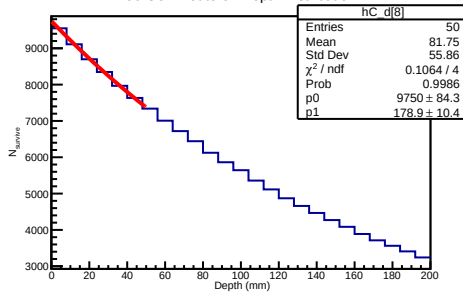
90 GeV Deuteron Depth Distribution
