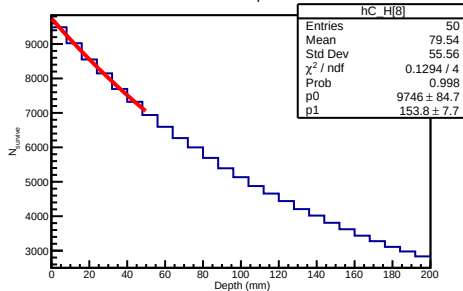
90 GeV Helium3 Depth Distribution
