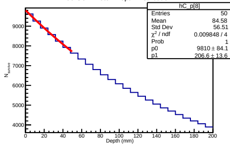
90 GeV Proton Depth Distribution
