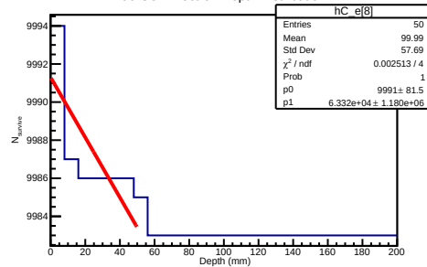
90 GeV Electron Depth Distribution
