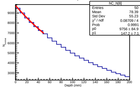
90 GeV Helium4 Depth Distribution
