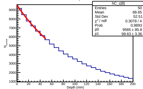
90 GeV Carbon Depth Distribution
