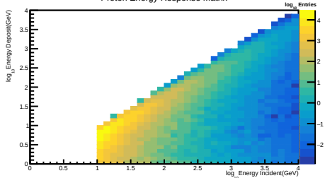
Proton Energy Response Matrix
