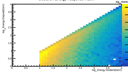
Deuteron Energy Response Matrix
