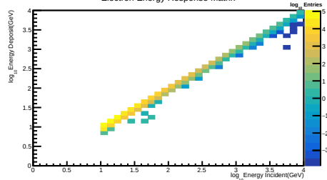
Electron Energy Response Matrix
