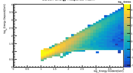
Carbon Energy Response Matrix
