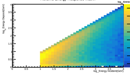
Helium3 Energy Response Matrix
