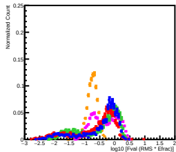
log10 [Fval (RMS * Efrac)] Distribution in L1
