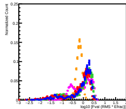
log10 [Fval (RMS * Efrac)] Distribution in L2
