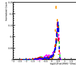
log10 [Fval (RMS * Efrac)] Distribution in L4
