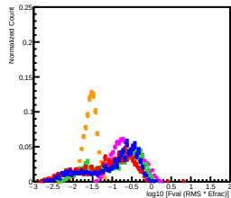
log10 [Fval (RMS * Efrac)] Distribution in L0
