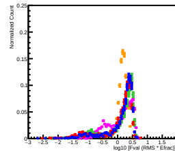
log10 [Fval (RMS * Efrac)] Distribution in L3
