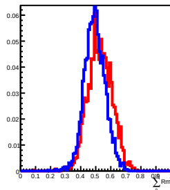
100 GeV incident in L11
