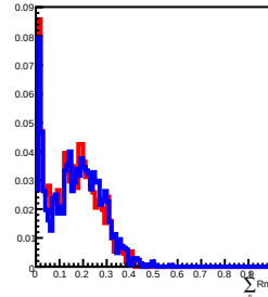
20 GeV incident in L7
