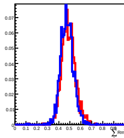
20 GeV incident in L11
