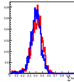
20 GeV incident in L12
