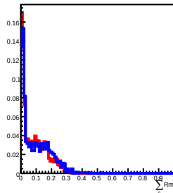
20 GeV incident in L6
