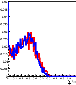
300 GeV incident in L10
