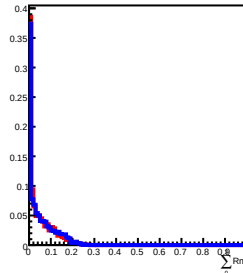
300 GeV incident in L7
