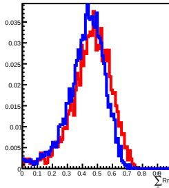
300 GeV incident in L13
