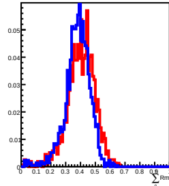
30 GeV incident in L12
