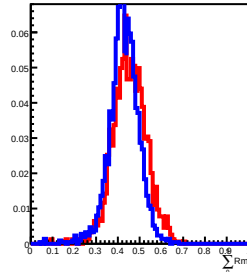
30 GeV incident in L9
