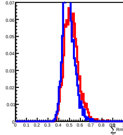
30 GeV incident in L13
