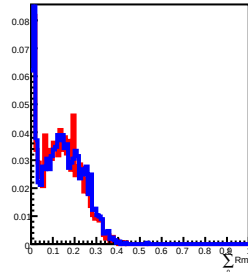
30 GeV incident in L7
