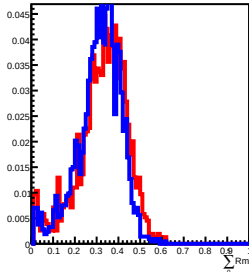
30 GeV incident in L10
