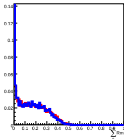
400 GeV incident in L9
