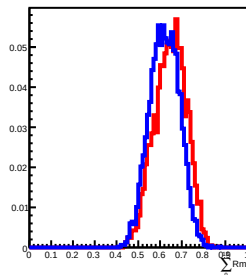
400 GeV incident in L13
