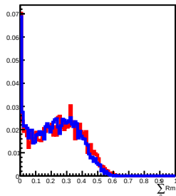
400 GeV incident in L10
