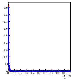
400 GeV incident in L5
