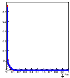
400 GeV incident in L6
