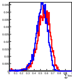
400 GeV incident in L10
