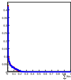
400 GeV incident in L7
