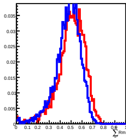
400 GeV incident in L9
