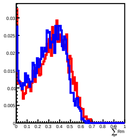
400 GeV incident in L11
