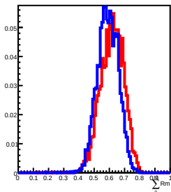
400 GeV incident in L12
