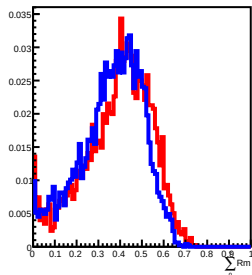
400 GeV incident in L12
