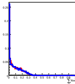
400 GeV incident in L8
