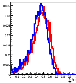
400 GeV incident in L13
