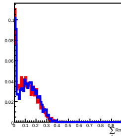
40 GeV incident in L7
