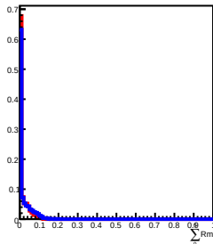
40 GeV incident in L5
