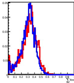
40 GeV incident in L10
