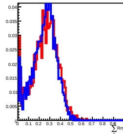
40 GeV incident in L9
