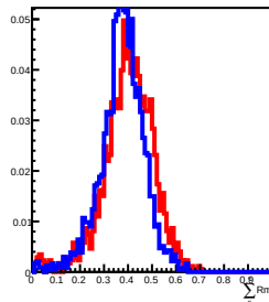
40 GeV incident in L12
