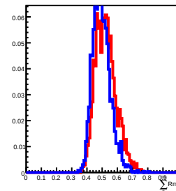
40 GeV incident in L13
