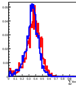
40 GeV incident in L11
