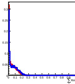
40 GeV incident in L6
