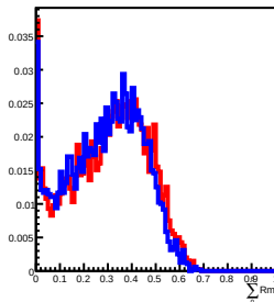
500 GeV incident in L11
