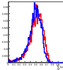
500 GeV incident in L9
