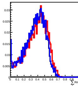
500 GeV incident in L12
