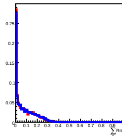
500 GeV incident in L8
