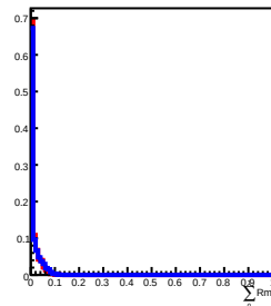
500 GeV incident in L6
