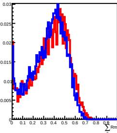
700 GeV incident in L12
