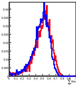
700 GeV incident in L9
