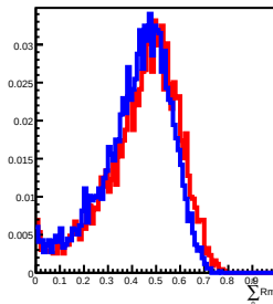
700 GeV incident in L13
