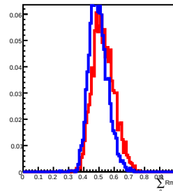
70 GeV incident in L12
