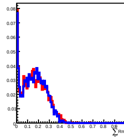
70 GeV incident in L8
