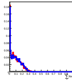
70 GeV incident in L7
