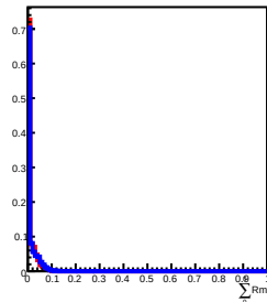
70 GeV incident in L5
