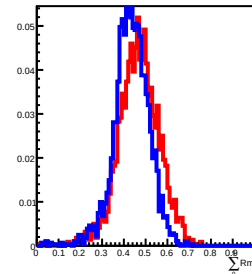
70 GeV incident in L9
