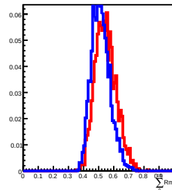
70 GeV incident in L13
