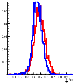
70 GeV incident in L10
