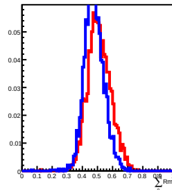
70 GeV incident in L11
