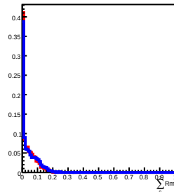
70 GeV incident in L6
