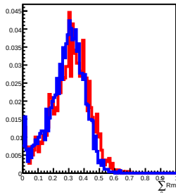
70 GeV incident in L10
