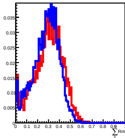
80 GeV incident in L10
