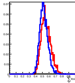
80 GeV incident in L13
