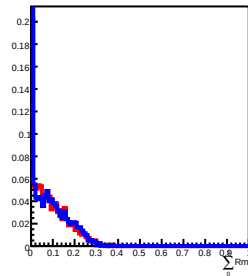
80 GeV incident in L7
