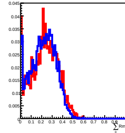
80 GeV incident in L9
