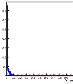
80 GeV incident in L5
