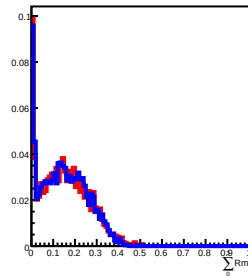
80 GeV incident in L8
