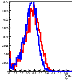
80 GeV incident in L11
