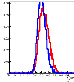
80 GeV incident in L12
