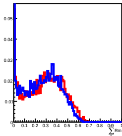
900 GeV incident in L11
