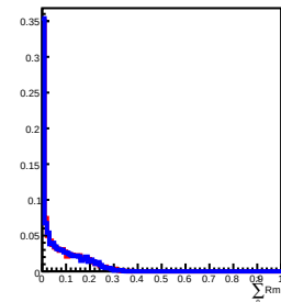
900 GeV incident in L8
