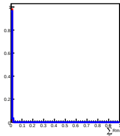
900 GeV incident in L5
