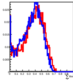
900 GeV incident in L12
