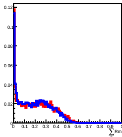
900 GeV incident in L10
