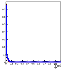
900 GeV incident in L6
