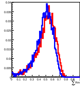
900 GeV incident in L9
