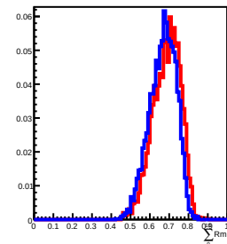
900 GeV incident in L13
