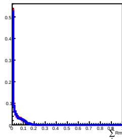
900 GeV incident in L7
