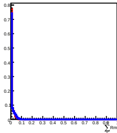
90 GeV incident in L5
