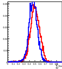
90 GeV incident in L10
