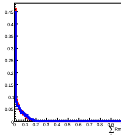
90 GeV incident in L6
