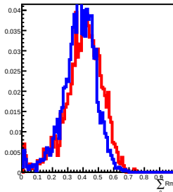
90 GeV incident in L12
