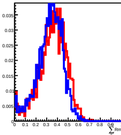
90 GeV incident in L11
