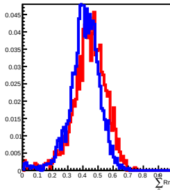
90 GeV incident in L13
