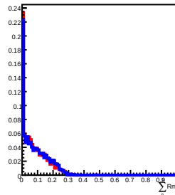
90 GeV incident in L7
