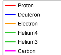
IncidentParticle 10GeV
