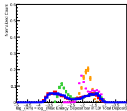
300 GeV incident in L1
