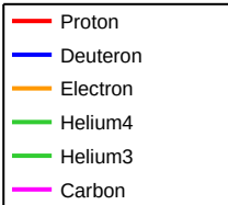
IncidentParticle 300GeV
