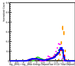
300 GeV incident in L3
