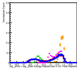
300 GeV incident in L2
