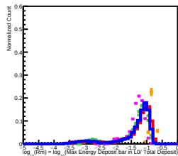
300 GeV incident in L4
