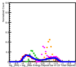
800 GeV incident in L1
