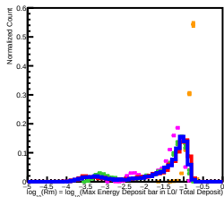
800 GeV incident in L4
